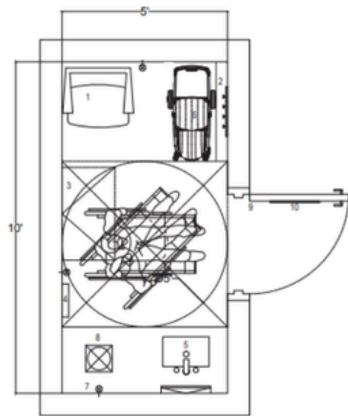
2-1 plan
